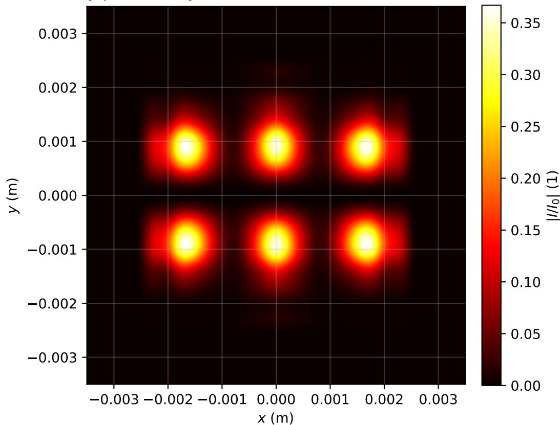
Intensity profile I(x, y, z = 3.742)/I_0 , P_{in}=3.0P_{cr} , artificial time
